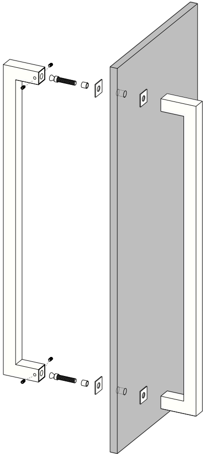
Axonometric View
