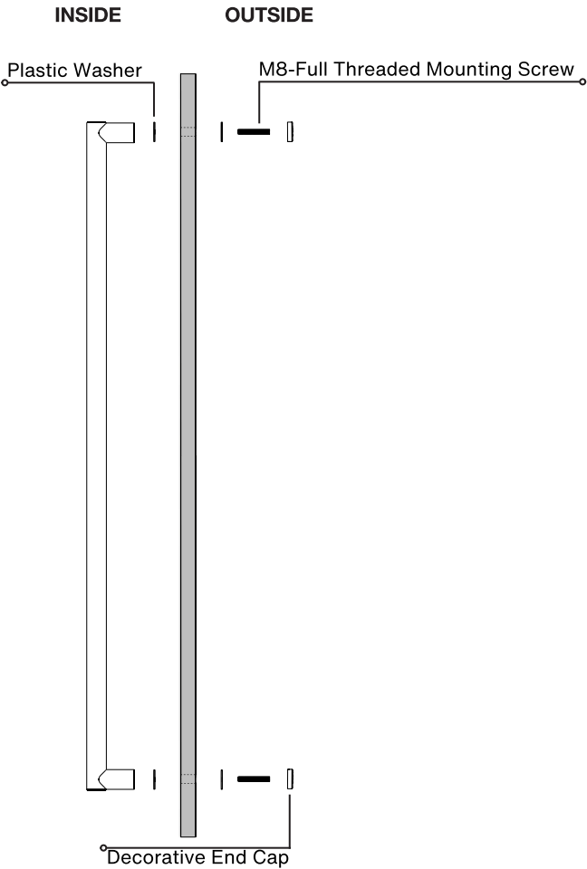
Top View
