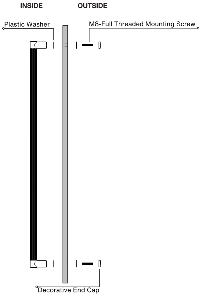
Top View
