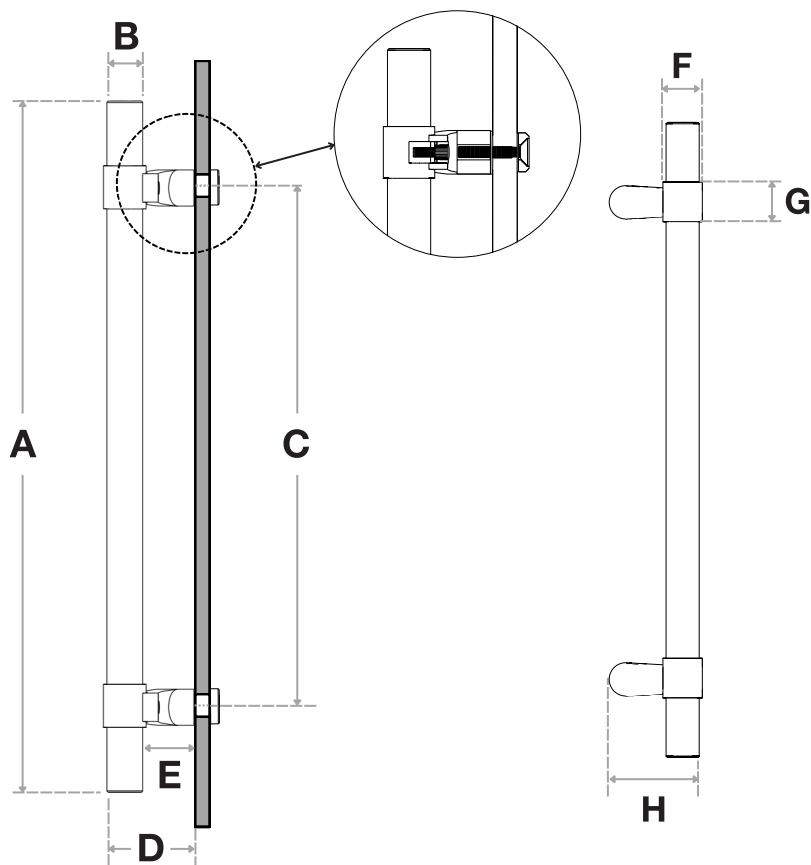
Side View
