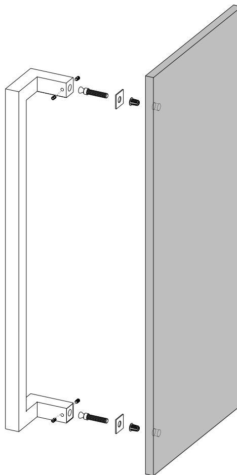
Axonometric View
