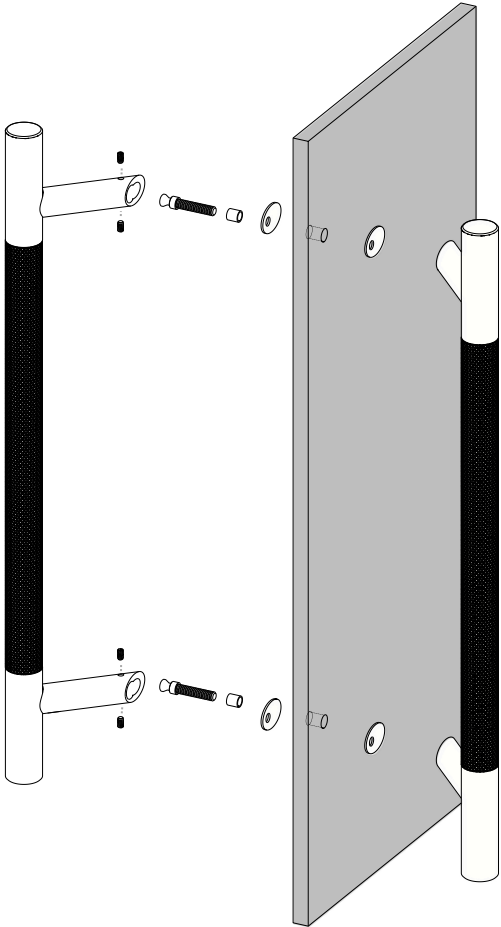
Axonometric View
