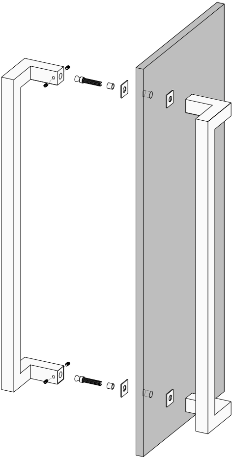
Axonometric View
