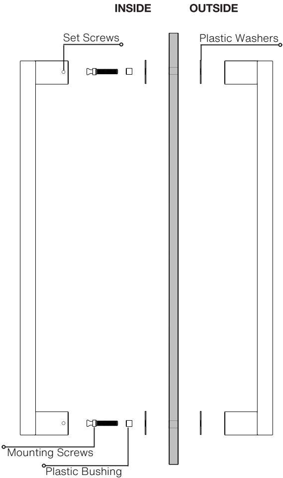
Side View
