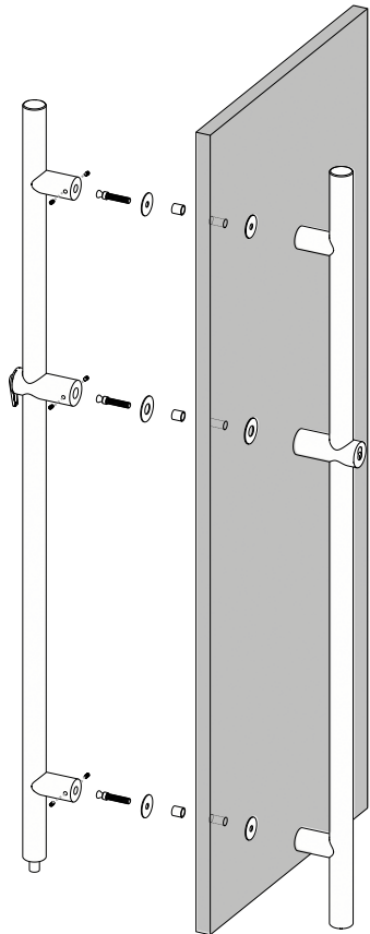
Axonometric View
