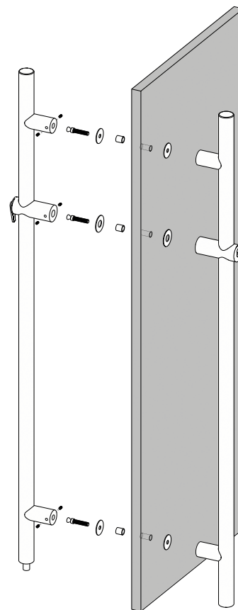
Axonometric View
