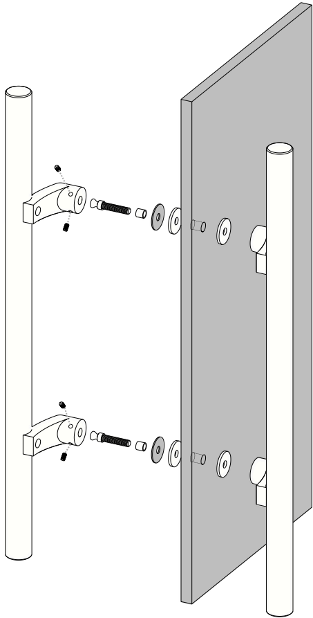
Axonometric View
